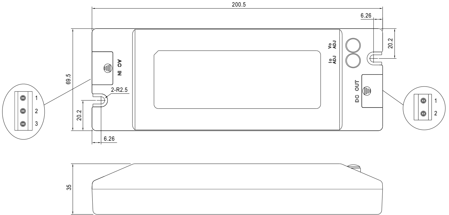
Terminal Pin No. Assignment (TB1): SWITCLAB MB310-75003
