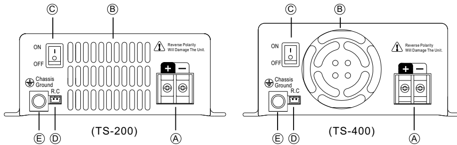
Figure 3.2: Rear Panel
